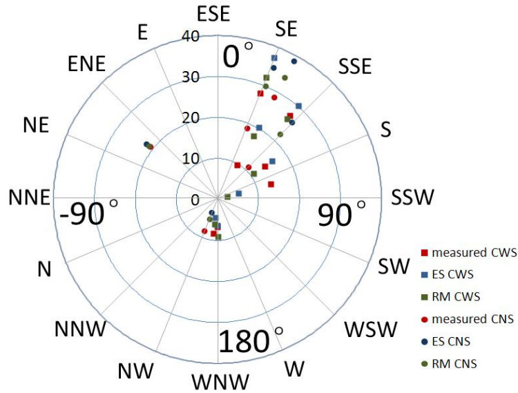
Figure 7. Measured and calculated ACR N (vol/h) in azimuth map
