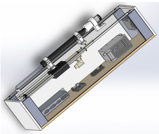
Figure 2: The new slide flute prototype
