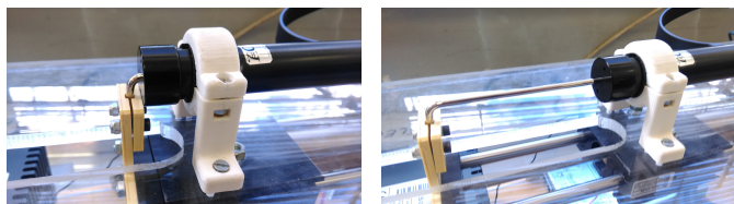
Figure 6: Left: position of the piston at the origin — Right: position of the piston at 10cm
