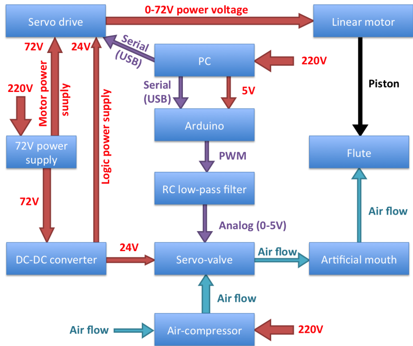
Figure 1: Synoptic diagram of the system — Red stands for power supply, purple for logic and cyan for air flow.
