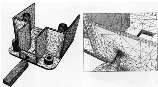
Figure 2. Example of a mold cavity meshing with sharp mesh refinement in the vicinity of the injection gate (Silva et al.[11])
