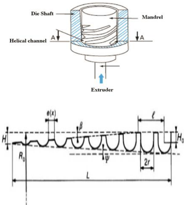
Figure 3. Geometry of a film-blowing die: (top) overall view; (bottom) cut in the vertical plane
