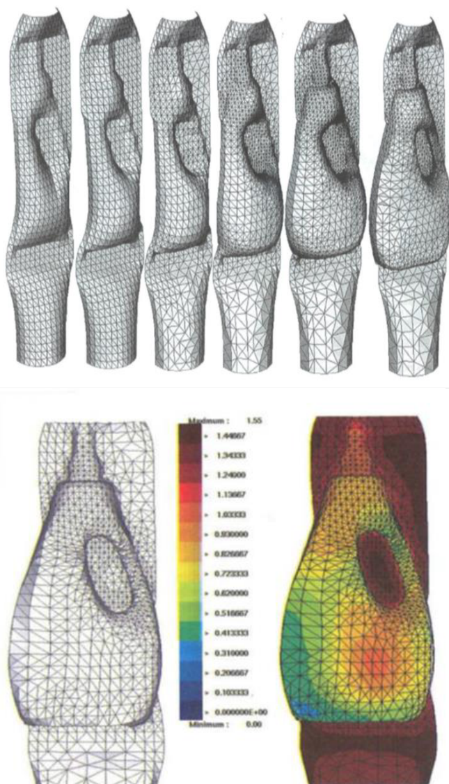
Figure 8. (top) Shape and meshing of the membrane at different steps of simulation of the extrusion; (bottom) Final mesh and thickness distribution in the bottle (Bellet et al.[34])
