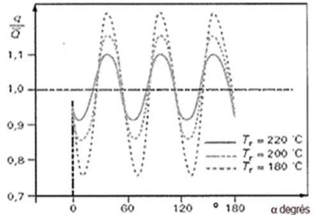
Figure 5. Influence of the thermal regulation of the die shaft on the polymer flow distribution at film-blowing die exit., q is the local flow along the circumference of the die , \bar{Q} is the average flow rate ( Vergnes et al.[12];Agassant and Vergnes [13])
