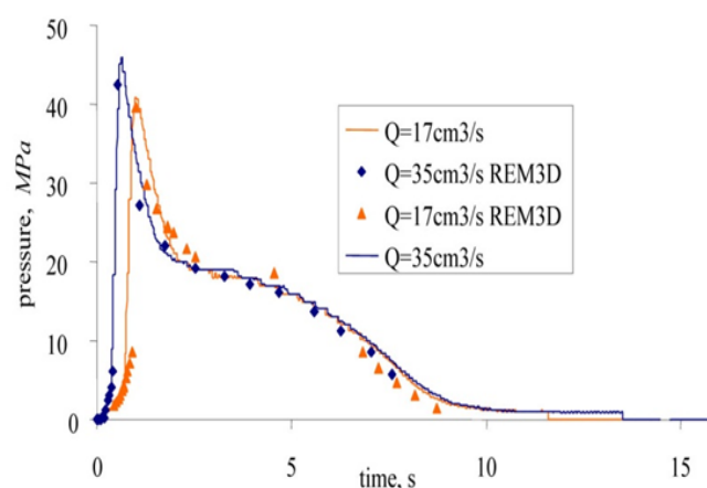
Figure 7. Pressure as a function of time in the cavity during the entire injection cycle for two different flow rates, the polymer is a polystyrene (Silva et al.[11]).
