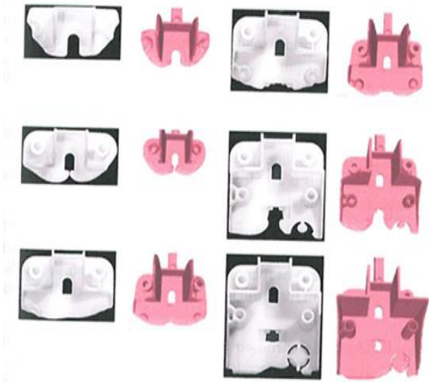
Figure 6. Computed (on the right in each column) and experimental (on the left in each column) short shots for the filling of the cavity presented Figure 2 (Silva et al.[11])
