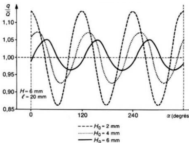
Figure 4. Influence of the initial depth of the channel H_0 on the polymer flow distribution at film-blowing die exit., q is the local flow along the circumference of the die , \bar{Q} is the average flow rate ( Vergnes et al.[12];Agassant and Vergnes [13]).
