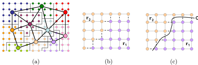
Fig. 2. (a) A region adjacency graph. (b) The set of nodes of the pixel graph considered to compute boundary properties between two regions, with a V_4 adjacency system. (c) A curve crossing the edges of the boundary between two regions r_1 and r_2 .
