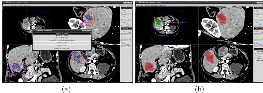
Fig. 4. Snapshot of the graphical user interface of our software. (a) Interactive marker drawing. (b) Visualization of a segmented data set.
