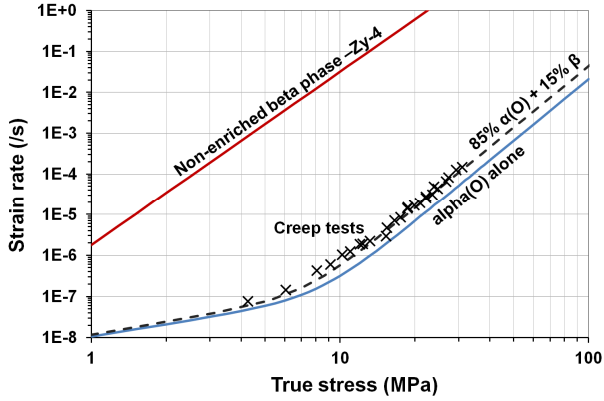
Fig. 7. Creep test results (symbols) and viscoplastic flow rules (lines), all determined in uniaxial tension along the tube axis at 900°C.
