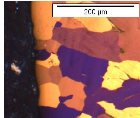
Fig. 3. Optical micrograph of an oxidized, then homogenized sample containing 2 wt% of oxygen. Same orientation as in Figure 1, outer surface on the left.
