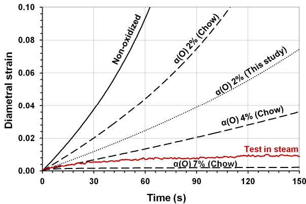
Fig. 11. Creep test in steam (red line) and creep simulations in an inert atmosphere for a 20-μm-thick alpha(O) layer with various oxygen contents (grey lines) – Zy-4 at 1100°C under 5 bar.
