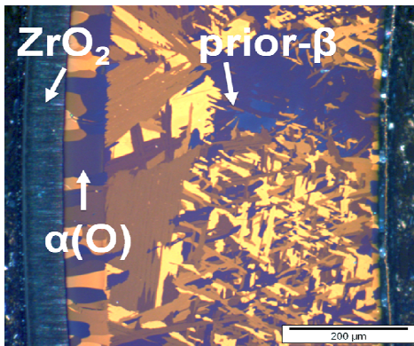
Fig. 1. Optical micrograph of a Zy-4 cladding after creep test in steam at 1100°C for 10 min. Outer surface on the left, tube axis perpendicular to the image.
