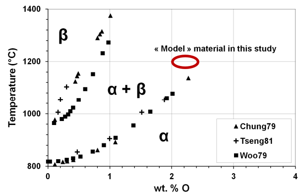
Fig. 4. Zircaloy-4 – oxygen isopleth from the equilibrium phase diagram 9,14,15 . The oxygen content and homogenization temperature are indicated with a red ellipse.
