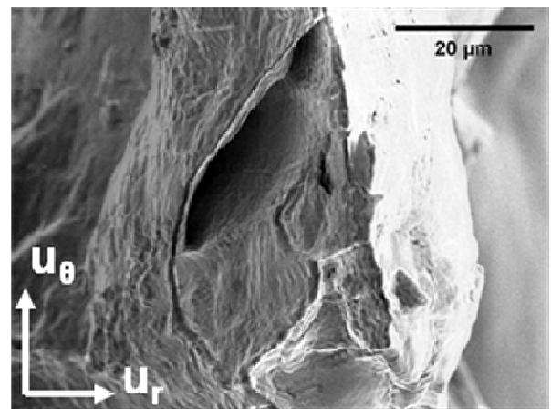
Fig. 5. SEM micrograph of the fracture surface of the 2 – 2.5 wt% oxygen enriched-material broken at 1000^\circ\text{C} .
