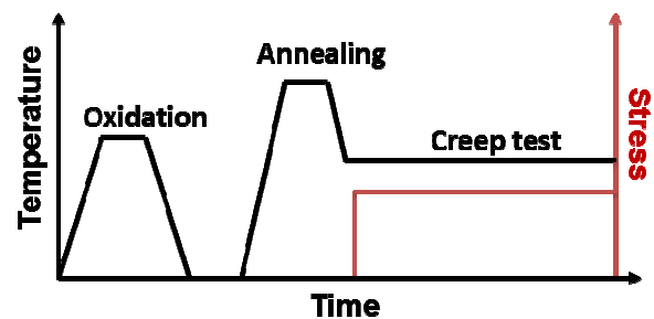
Fig. 2. Scheme of the thermal-mechanical history of the oxygen-enriched creep specimens.
