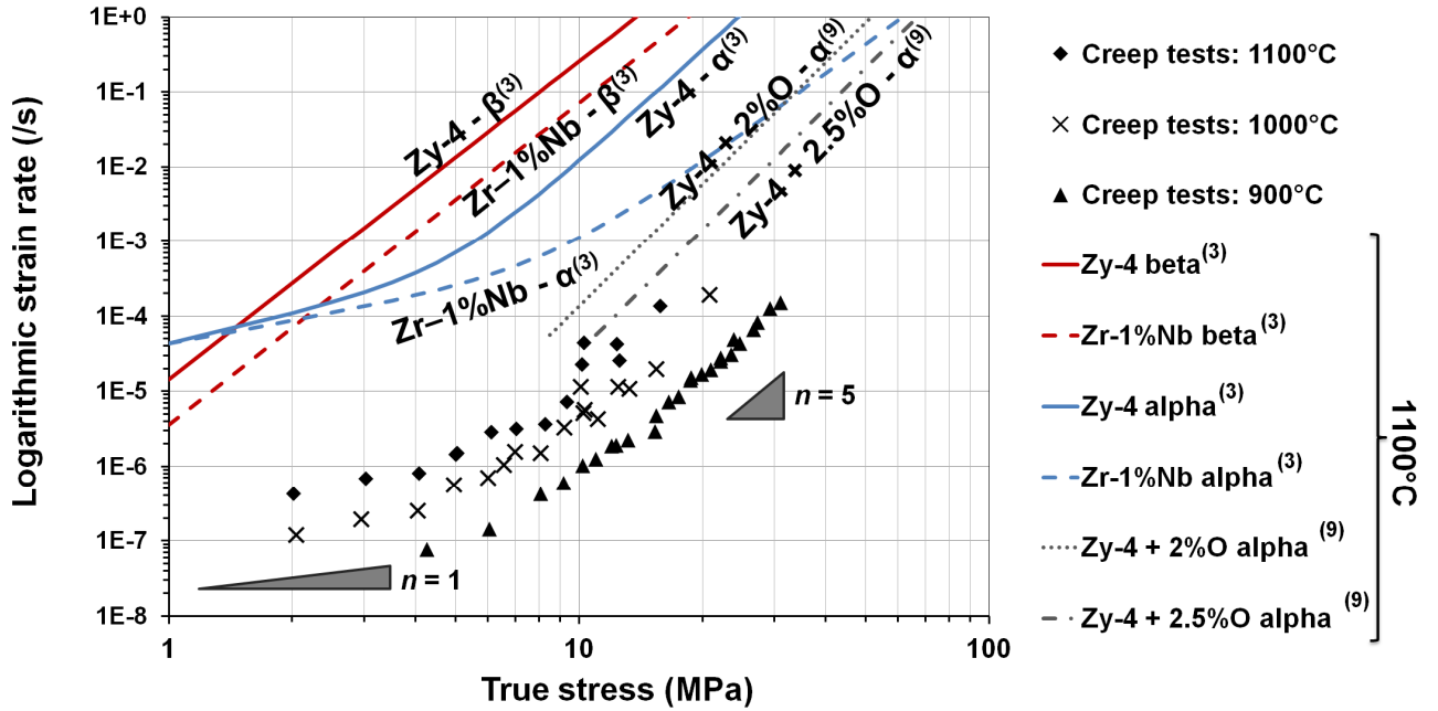
Fig. 6. Stress dependence of the strain-rate: present experimental data (symbols) for oxygen-enriched material, predictions at 1100°C for zirconium alloys which are non-enriched 3 (color lines) or enriched with oxygen 9 (grey lines).
