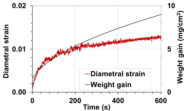
Fig. 8. Predicted weight gain based on data from Brachet et al. 11 versus time, together with creep strain of Zy-4 at 1100°C and 5 bar of internal pressure in steam.
