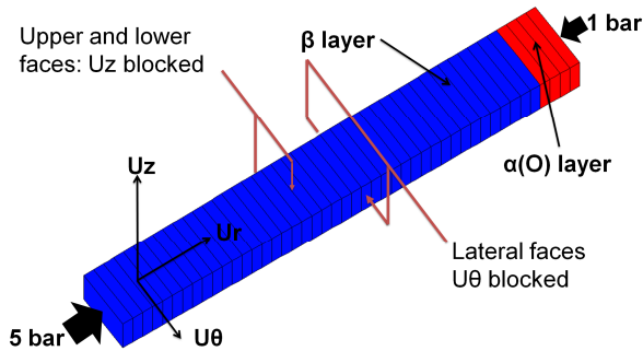
Fig. 9. Mesh, loading and boundary conditions used in FE simulations of internal pressure loading at 1100°C.
