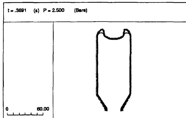
Fig. 12. Intermediate bottle shapes.
