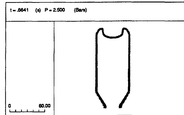
Fig. 12. Intermediate bottle shapes.
