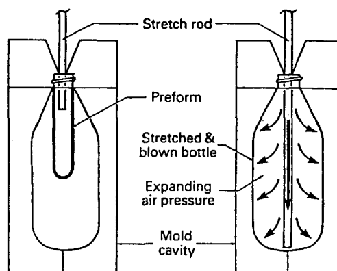
Fig. 1. Description of the stretch/blow molding step.
