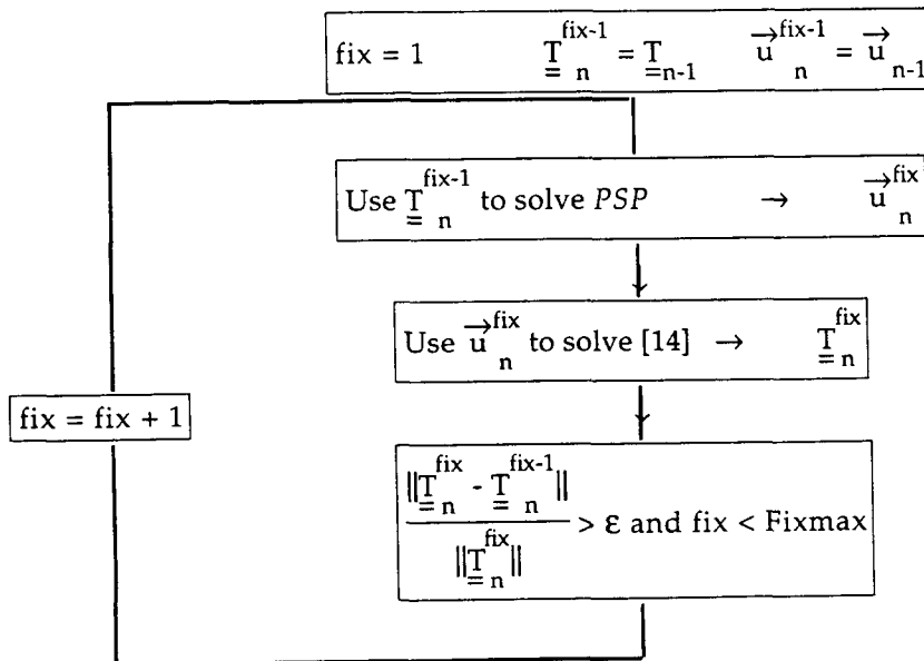
Fig. 3. Fixed-point algorithm.
