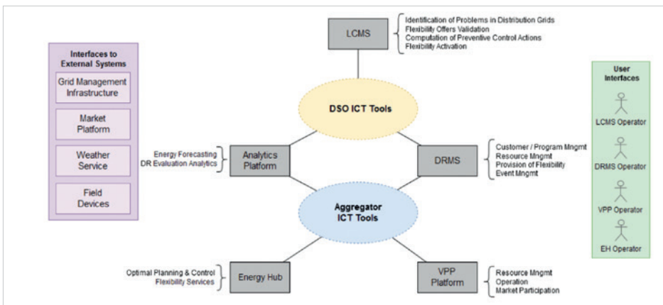
Figure 14: The SmarterEMC2 High Level Conceptual Architecture
