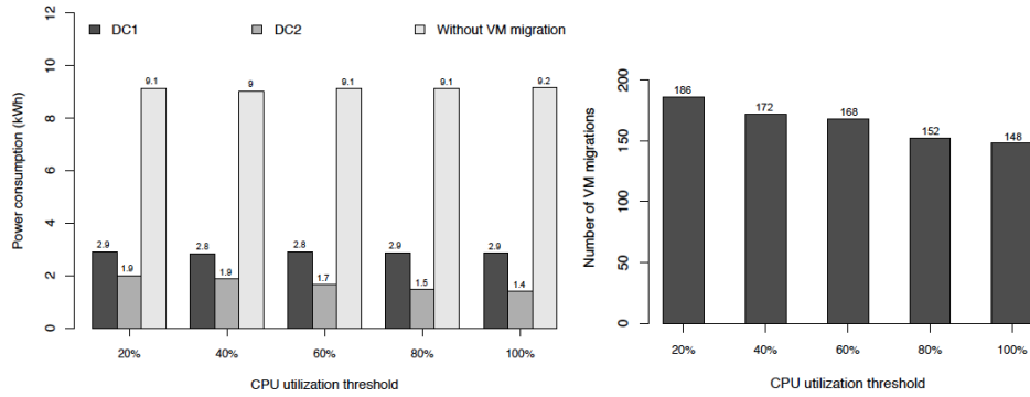
(a) Power consumption of the data centers with and (b) Number of VM migrated from DC1 to DC2 without the FAP approach using the FAP approach
