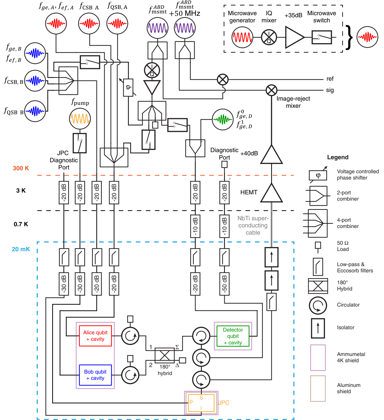
FIG. 5. Detailed experimental setup. The experiment (bottom) was cooled down on the base stage ( < 50 \text{ mK} ) of a dilution refrigerator. Input lines carrying signals to the systems were attenuated and filtered using commercial low-pass filters and homemade lossy Eccosorb filters. The room-temperature electronics used to produce and shape the input signals are shown at the top of the figure. The basic setup to produce shaped signals was a microwave generator driving an IQ mixer followed by an amplifier and finally a switch to gate the signal (box in top-right corner). The signals were shaped by channels from four arbitrary waveform generators (AWGs) (not shown), which also provided the digital markers for the switches. Copies of this setup (denoted by the shorthand notation of a circle with a shaped pulse) were used to generate the drive signals (color-coded) for three modules: Alice (red), Bob (blue), and the detector (green). The Alice and Bob modules had four inputs each: the cavity readout tone, the qubit signals, and the pair of sideband pulses for photon generation. On the other hand, the detector module had two inputs: the cavity readout tone and the qubit signals. All the modules were read out using a single output line that had multiple stages of amplification. High-fidelity single-shot readout was enabled by the JPC amplifier. The output signals were downconverted and then digitized and demodulated along with a room-temperature reference copy.
