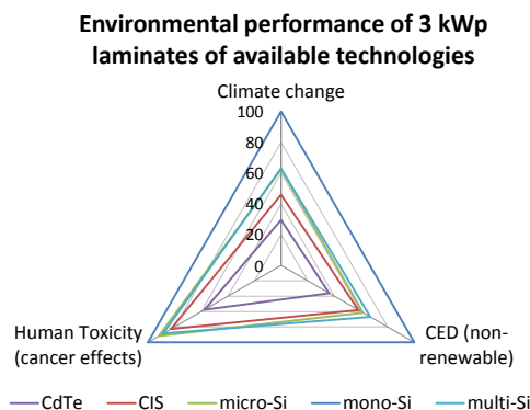
Figure 4: Comparative environmental performance of 3 kWp laminates of current PV technologies available in the Web-Service, operating at 45° inclination and south orientation
