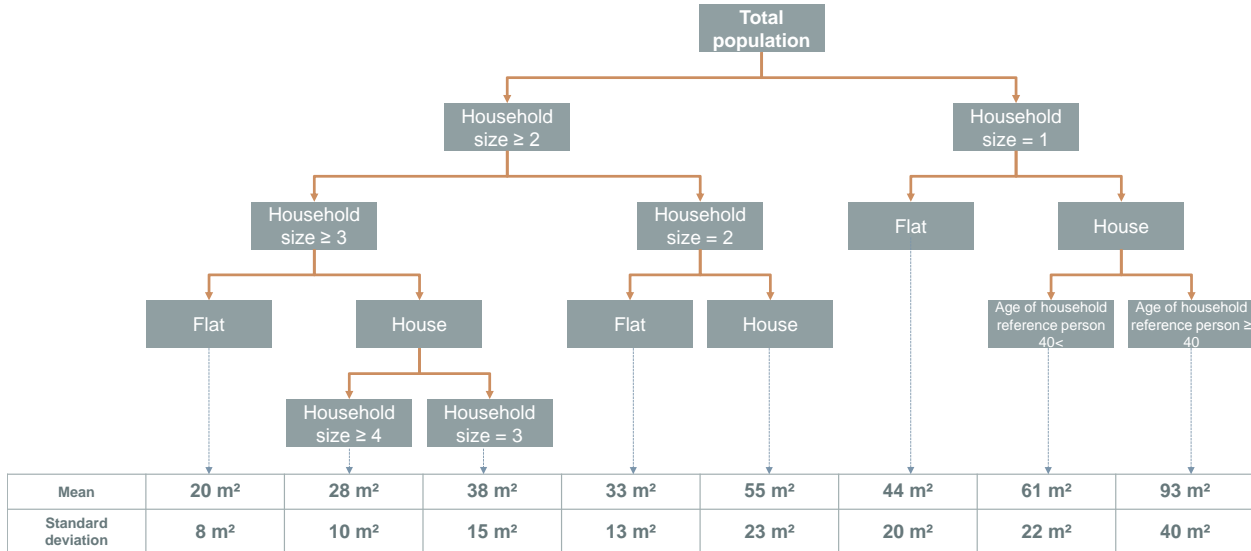
Figure 5. Regression tree related to the space floor per person and its associated matrix. Data source: Housing survey 2006 for France.
