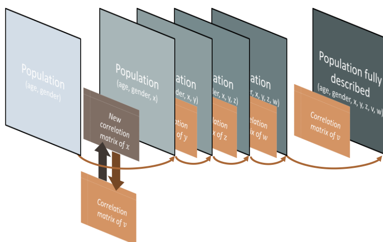
Figure 6. Illustration of the process of changing matrices. In this generic case, the correlation matrix of x is changed.
