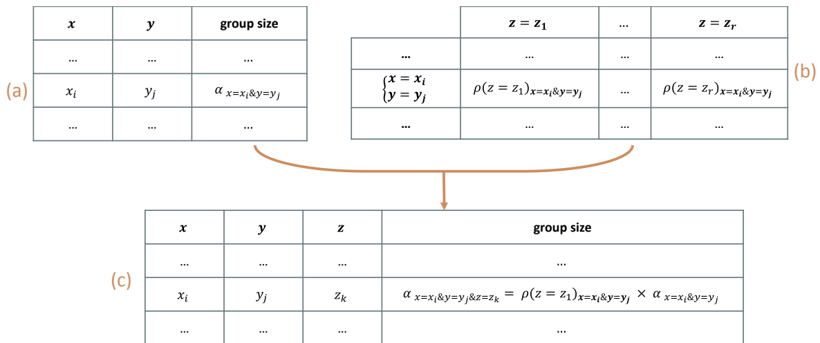
Figure 4 : Example of adding a variable to the statistical model.
