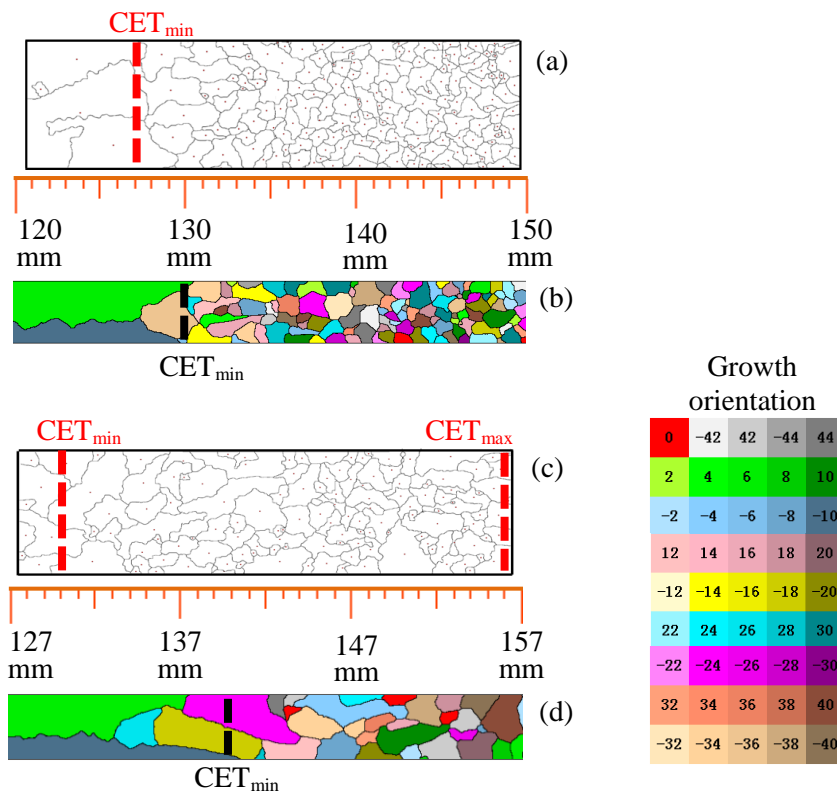
Figure 3. Comparisons of grain structures on section L4 (b) and (d) simulated using CAFE model with (a) and (c) EBSD measurements. (a) and (b) FM1 (refined Al - 7 wt% Si alloy, V_2 = 0.2 mm s^{-1} ); (c) and (d) FM5 (refined Al - 7 wt% Si alloy, V_2 = 0.01 mm s^{-1} ).
