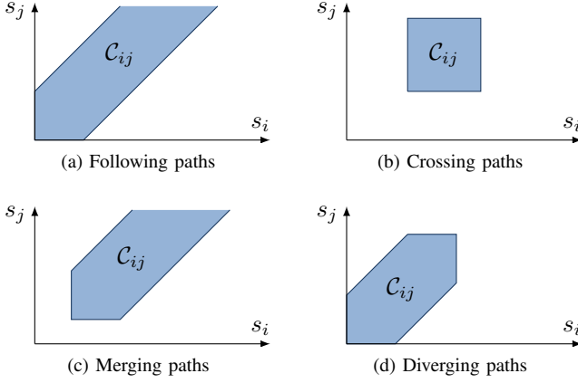
Fig. 2. Possible bounding polygons for the collision set between two conflicting robots i and j . The edges of C_{ij} are straight lines with equations s_i = A , s_j = B or |s_i - s_j| = C where A, B, C are constants.
