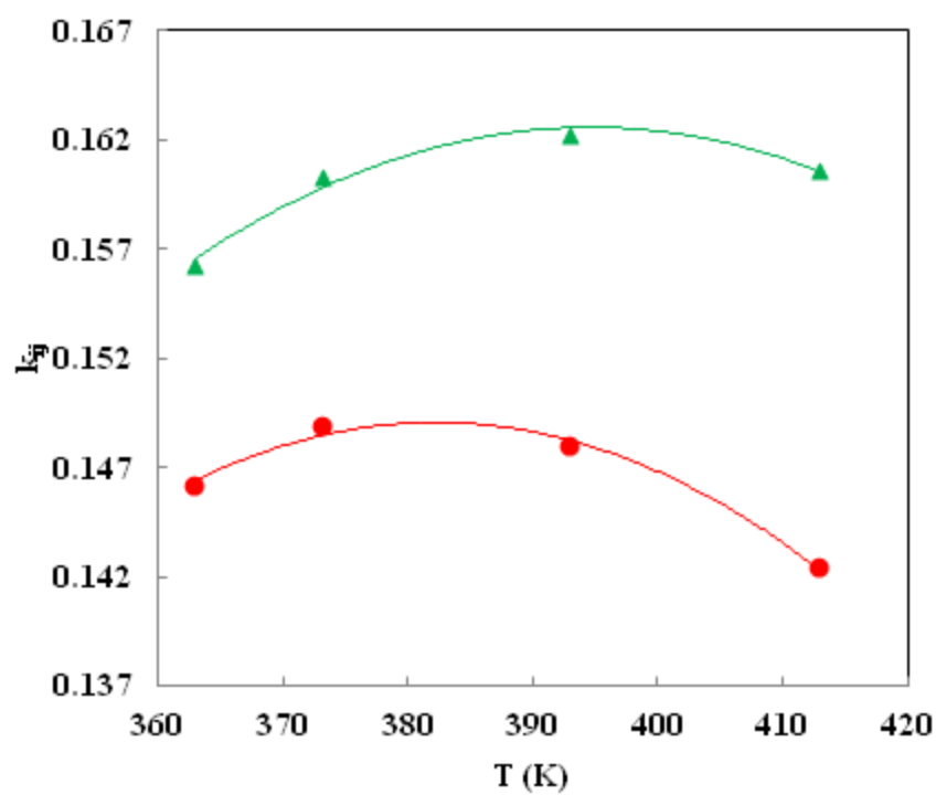
Fig. A.47 - k_{ij} as a function of temperature: isopentane + R-245fa. (●) NEoS; (▲) PR-EoS.
