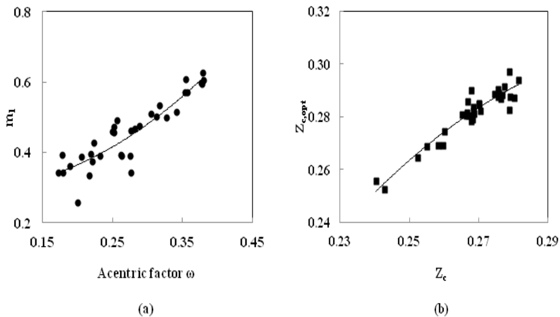
Fig. 22 - Correlations obtained with the NEoS. (a): the m_1 parameter as a function of the acentric factor \omega (coefficient of determination R^2 = 0.82 ); (b): the optimized critical compressibility factor Z_{c,opt} as a function of the experimental critical compressibility factor Z_c (coefficient of determination R^2 = 0.89 ).
