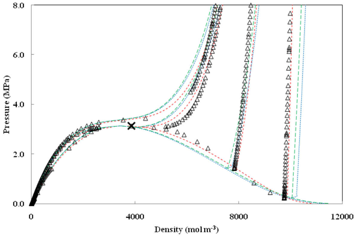
Fig. 25 - P- \rho diagram for R-1216.
