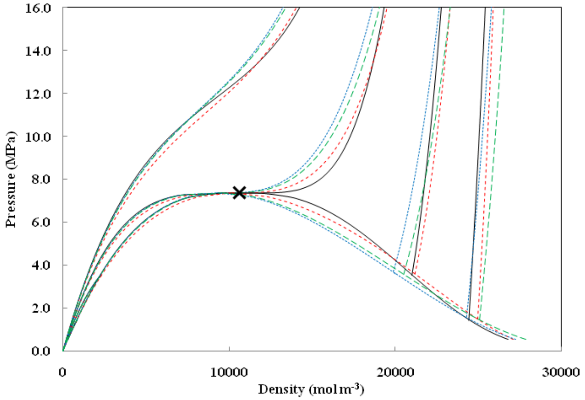
Fig. 26 - P- \rho diagram for CO 2 . (—) REFPROP; (×) Critical Point: REFPROP ( T_c=304.13\text{K} ); (- - -) N-EoS; (.....) PT-EoS; (- - -) PR-EoS. Out of saturation: T_r = 0.8, 0.9, 1.0 , and 1.1 .
