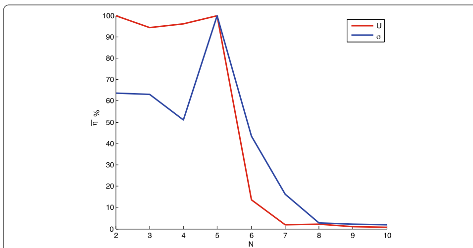
Fig. 8 Convergence of the approximation errors on simulation outputs, for \mu = \mu^1 and over the last cycle of loading, according to the infinite norm. The curve in red is related to the relative error on displacements at points A, B and C . The blue curve is related to the stresses in the numerical inclusion
