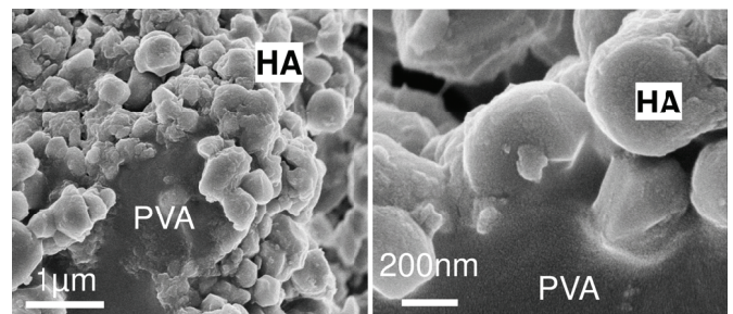
Fig. 10 SEM views of HA/PVA interface within a crater
