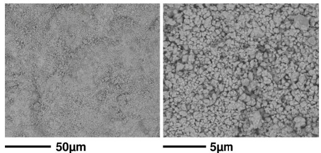
Fig. 6 Top surface SEM-BSE views of calcined HA coatings on SB Ti-6Al-4V (T=230 °C, P=1.0 MPa)
