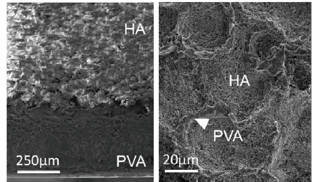
Fig. 9 SEM fractographic and top surface views in the centre (left) and at the boundary (right) of the HA track
