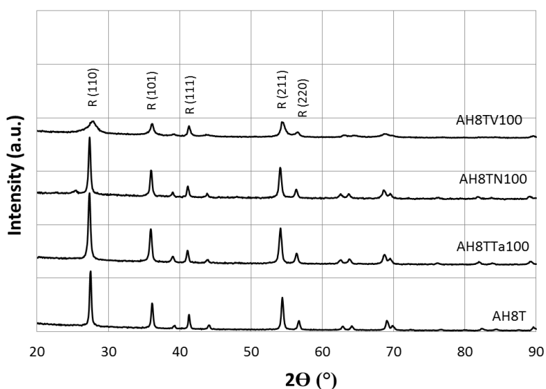
Figure 1. XRD of pure and doped \text{TiO}_2 aerogels calcined 5 h at 800^\circ\text{C} in flowing \text{H}_2/\text{N}_2 (5 vol.%)
