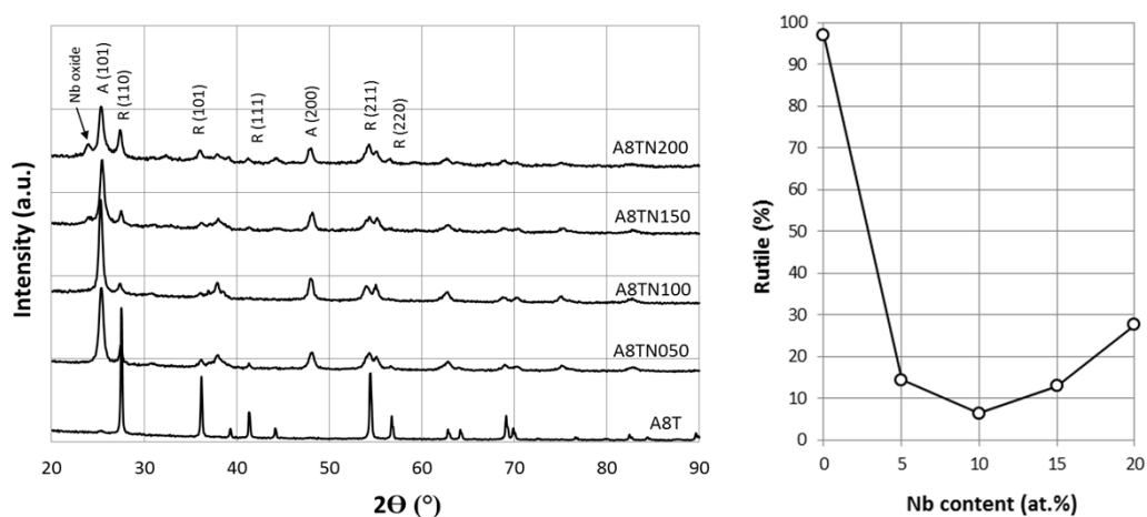
Figure 3. XRD of Nb doped TiO 2 aerogels calcined in flowing air, 5 h at 800 °C (left) and evolution of rutile content vs Nb doping level (right)
