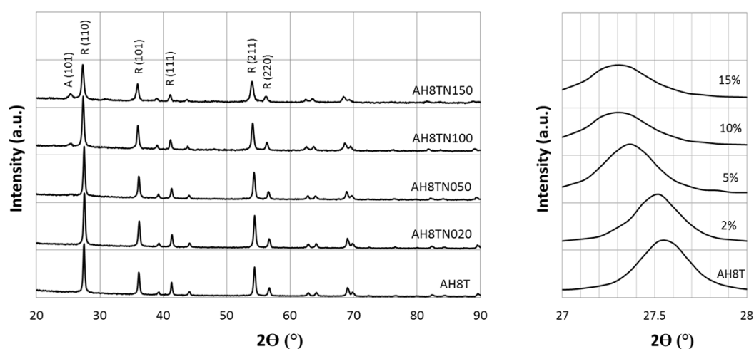
Figure 2. XRD of Nb-doped \text{TiO}_2 aerogels calcined 5 h at 800 °C in flowing \text{H}_2/\text{N}_2 (left) and R(110) peak shift (right) for different Nb contents.
