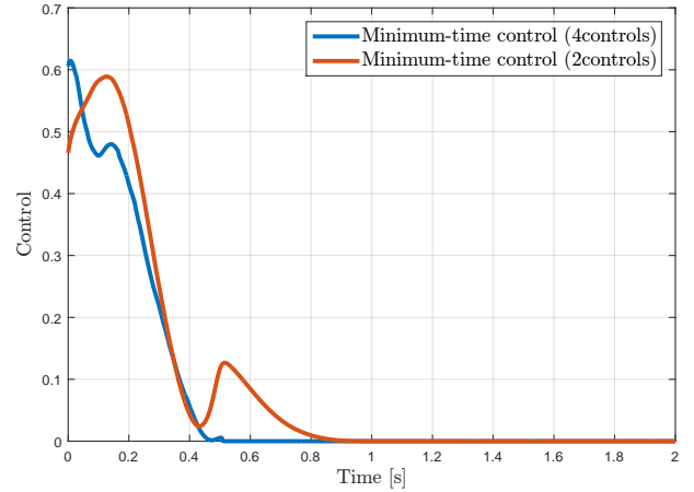
Fig. 5. Controller dynamics
