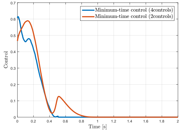
Fig. 5. Controller dynamics
