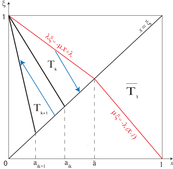
Fig. 3. Representation of the triangles \mathcal{T}_k
