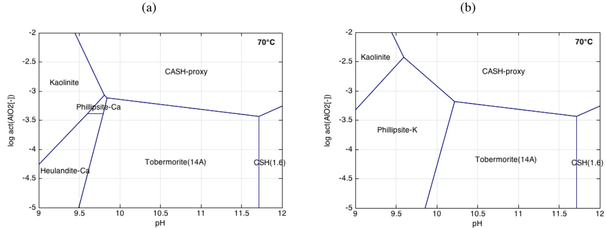
Fig. 14. Computed stability diagrams of Ca-Al-phases at 70°C without considering (a) and considering (b) Na-K ion activity ( \text{act. Ca}^{2+} = 10^{-3} , \text{act. Na}^+ = 10^{-2} , \text{act. K}^+ = 10^{-1} , [\text{H}_4\text{SiO}_4]_{\text{total}} = 10^{-3} molal).
