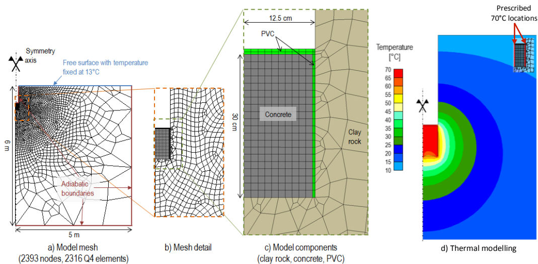
Fig. 2. Thermal modelling features: geometry, mesh and boundary conditions (a-b) and materials (c). Temperature field simulation (close-up view) after 1 year of heating at 70°C for the coil heating device (d)
