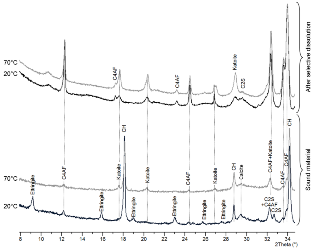
Fig. 1. XRD diagrams of the sound OPC paste at 20 and 70°C before and after selective dissolution. Selective dissolution facilitates detection of minor phases such as katoite.
