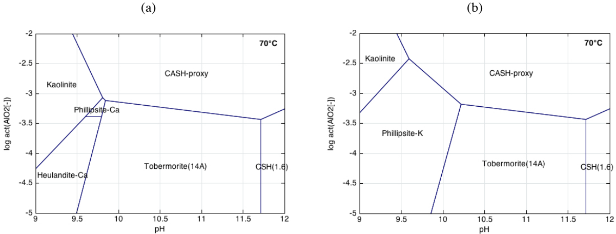
Fig. 14. Computed stability diagrams of Ca-Al-phases at 70°C without considering (a) and considering (b) Na-K ion activity (act. \text{Ca}^{2+} = 10^{-3} , act. \text{Na}^+ = 10^{-2} , act. \text{K}^+ = 10^{-1} , [\text{H}_4\text{SiO}_4]_{\text{total}} = 10^{-3} molal).
