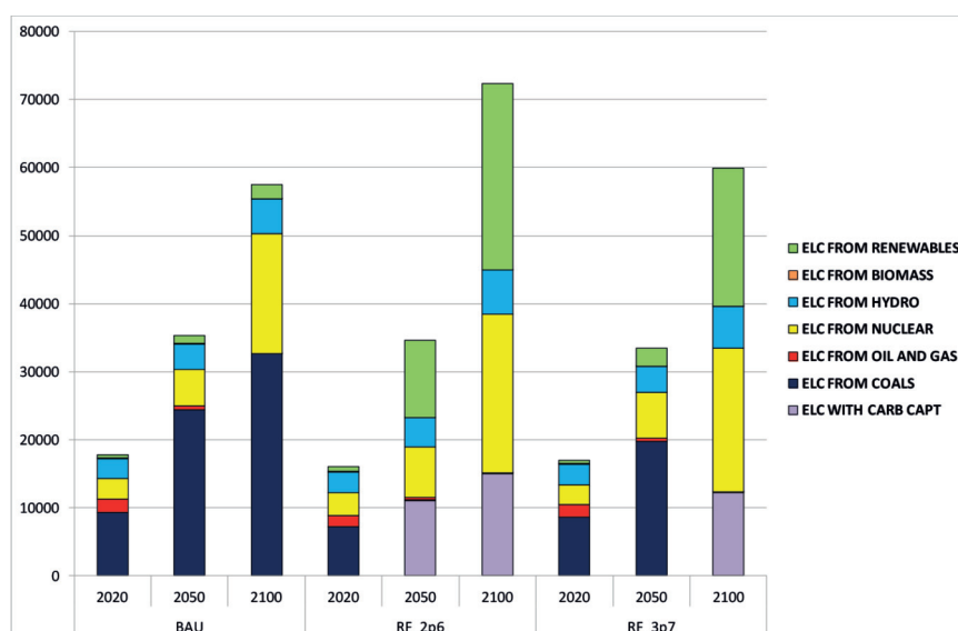
Figure 4: World power generation (TWh)
