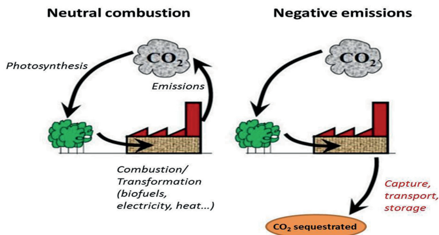
Figure 1: Negative emissions in the bioenergy lifecycle
