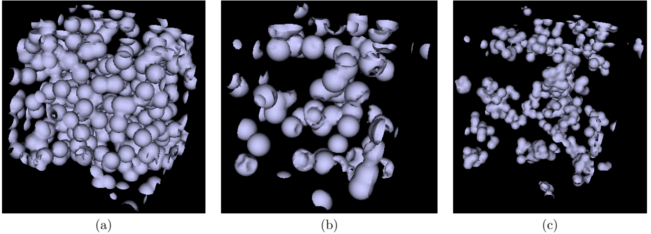
Figure 3: The three steps of the construction of the model: (a) exclusion polymer (Boolean model of spheres); (b) aggregates; (c) carbon black particles network ( v_e = 0.2 ; R_e = 30 nm; R_a = 60 nm; R_{cb} = 20 nm; simulated volume: (500 \text{ nm})^3 ).
