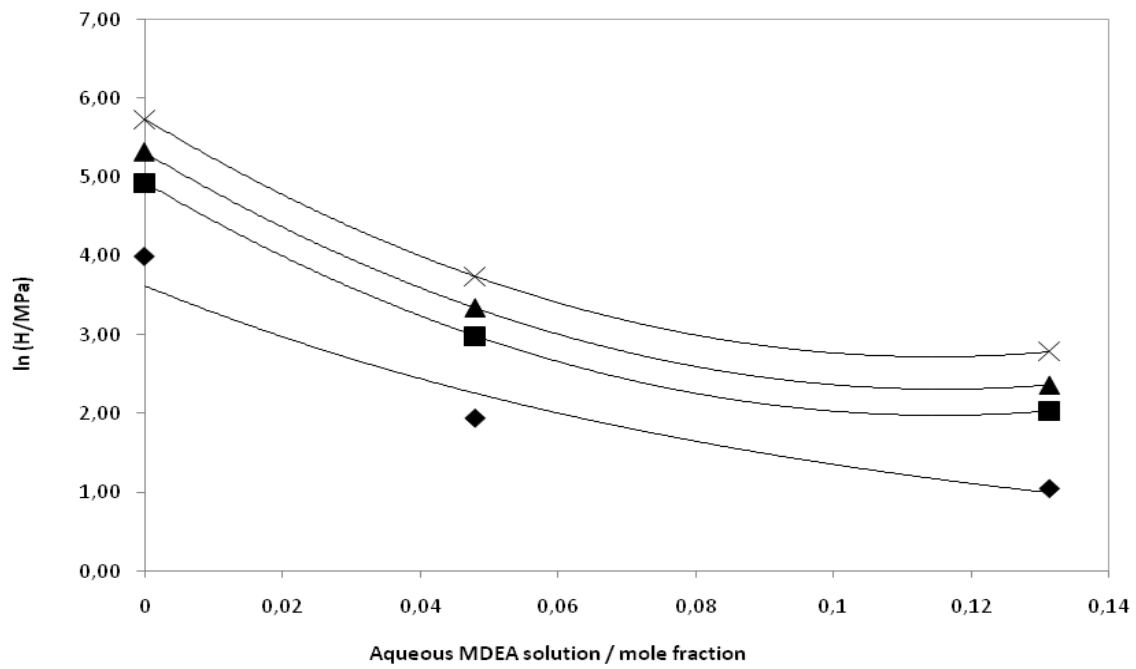
4 Figure 5. Tendency curves of Henry's Law Constant Logarithm for isobutyl mercaptan in 5 water and in various MDEA mole fractions at different temperature ◆ 298K ■ 323K ▲ 6 333K × 348K.
