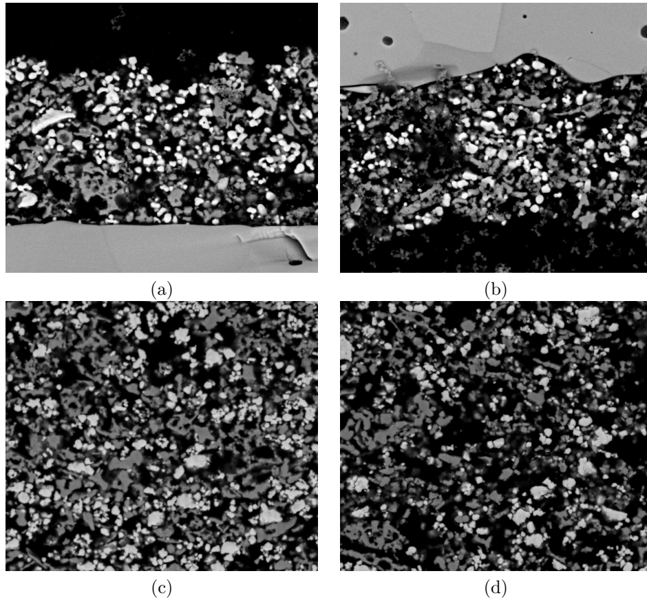
Figure 2: SEM images of symmetric cells 14 (a; b) and 29 (c; d) manufactured by CNR ISTECH. Images are 1024 pixels ( 12.7\ \mu\text{m} ) wide and 883 pixels ( 11\ \mu\text{m} ) height for a spatial resolution of 12.4\ \text{nm}/\text{pixel} (images: D. Masson). Images (a) and (c) show the layer on top of the electrolyte, and (b) and (d) on the bottom. Black: pores; white: GDC; dark-gray: LST. The electrolyte is visible in images (a) and (b).
