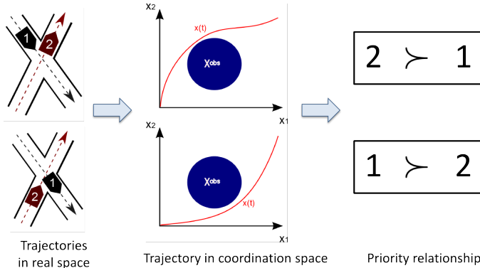
Fig. 1. An illustration of the concepts with 2 vehicles: real space, coordination space and priorities
