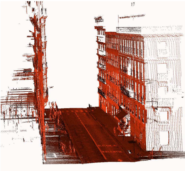
(a) Point cloud colored by the laser intensity.
