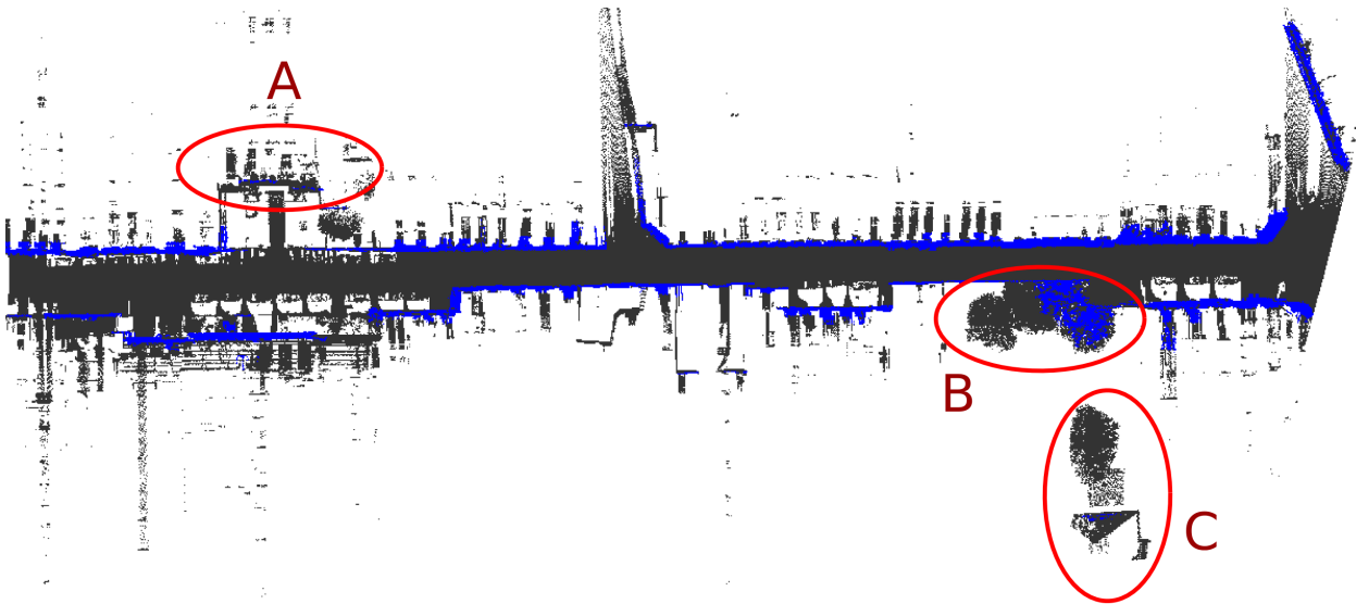
Figure 24. Façade segmentation result using the maximal elongation image on “Cassette_idclass.ply” file. Ground (gray), façades (blue). Input file taken from TerraMobilite/iQmulus database. Stereopolis II, IGN©. Errors are due to an incomplete detected façade (zone A) and a tree alignment connected to a low wall (zone B). Zone C corresponds to non-annotated points.
