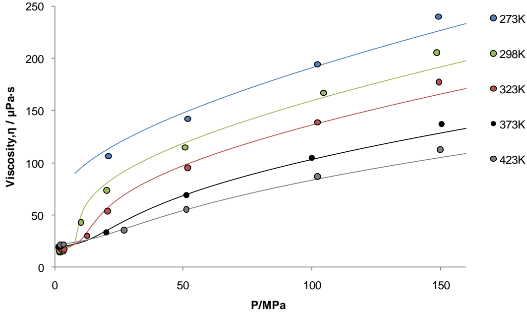
Fig. 2: Experimental (Chapoy et al. 2013) and predicted viscosity of a CO 2 -rich system (90%CO 2 , 5%O 2 , 2%Ar and 3%N 2 ).
