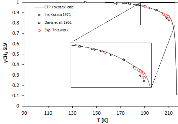
Figure 5. Comparison among literature data for the Ty SLV locus of the CH 4 -CO 2 mixture, experimental data obtained in this work and results obtained with the Yokozeki EoS [49] for SLV calculation.
