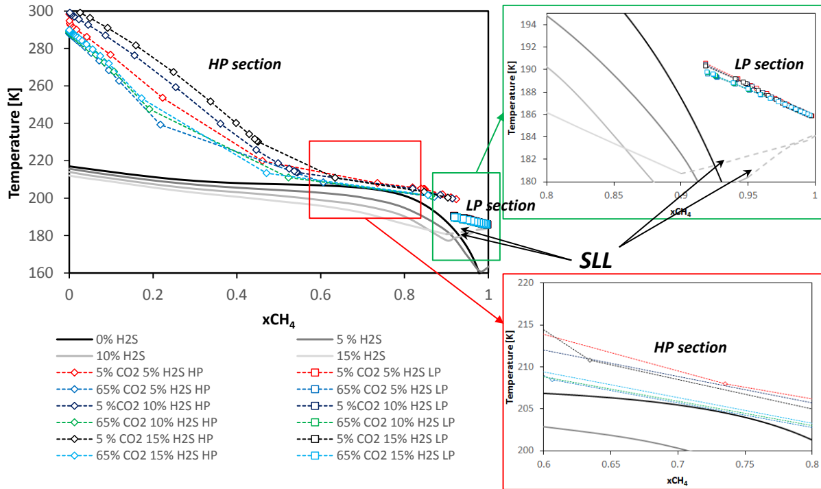
Figure 11. SLE lines at 50 bar for the ternary CH_4 - CO_2 - H_2S system and check of the possible formation of a solid phase in the process involving the ternary system.
