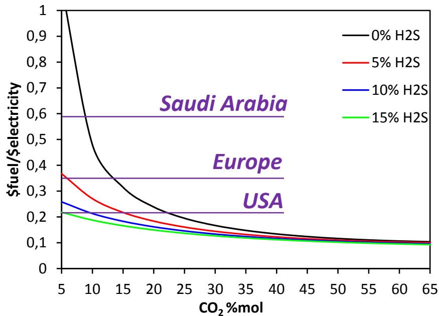
Figure 12. Breakeven point loci obtained as functions of costs of gas and electricity, and the acid gas contents in natural gas. Trade-off for different geographic areas is highlighted.
