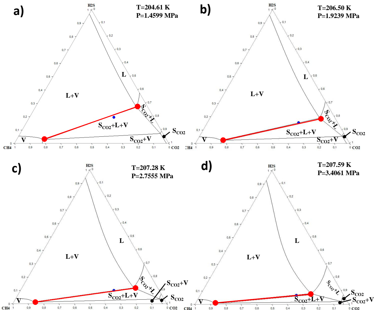
Figure 8. Phase equilibrium for the \text{CH}_4\text{-CO}_2\text{-H}_2\text{S} system. The graphs from a) to d) show the evolution of the phase diagram when progressive amounts of \text{H}_2\text{S} are added to a mixture of \text{CH}_4\text{-CO}_2 with a mole ratio of about 0.3/0.7. ●—●: experimental tie line for the ternary \text{CH}_4\text{-CO}_2\text{-H}_2\text{S} mixture; ●: global composition and —: model results. From a) to d) the \text{H}_2\text{S} molar fraction in the global composition is about: 0.20, 0.15, 0.10 and 0.05 respectively.
