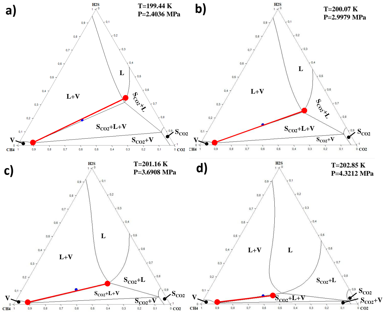
Figure 7. Phase equilibrium for the CH 4 -CO 2 -H 2 S system. The graphs from a) to d) show the evolution of the phase diagram when progressive amounts of H 2 S are added to a mixture of CH 4 -CO 2 with a mole ratio of about 0.4/0.6. ●—●: experimental tie line for the ternary CH 4 -CO 2 -H 2 S mixture; ●: global composition and —: model results. From a) to d) the H 2 S molar fraction in the global composition is about: 0.20, 0.15, 0.10 and 0.05 respectively.
