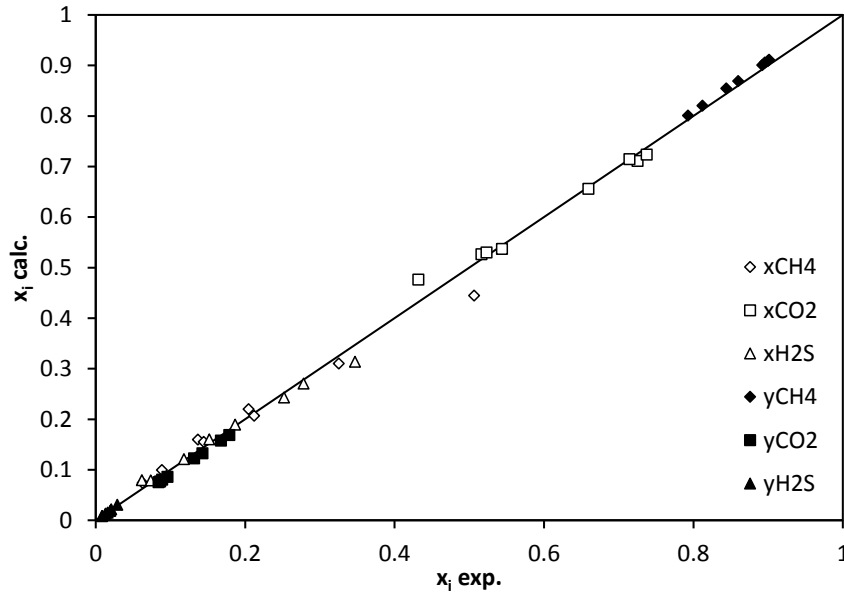
Figure 9. Model performances (Yokozeki, 2003 with binary interaction parameters obtained in this work) for the prediction of SLV composition for the ternary CH 4 -CO 2 -H 2 S mixture.
