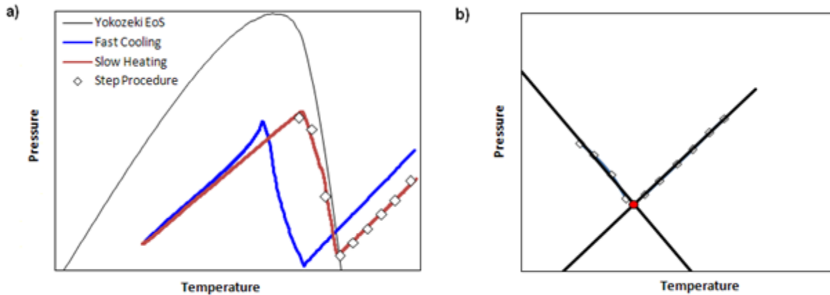
Figure 2. a) Definition of the experimental procedure and b) example of triple point calculation from PT data.
