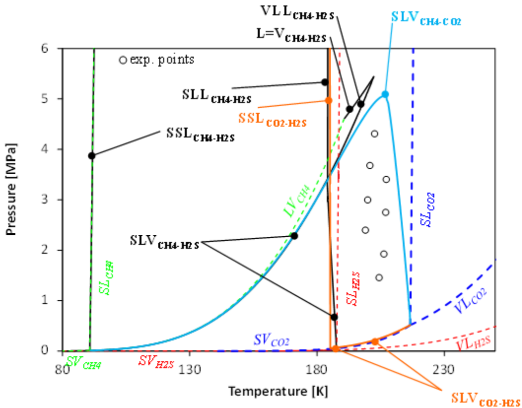
Figure 6. PT projections of the \text{CH}_4\text{-CO}_2 , \text{CO}_2\text{-H}_2\text{S} and \text{CH}_4\text{-H}_2\text{S} systems with experimental TP measurements for the \text{CH}_4\text{-CO}_2\text{-H}_2\text{S} system. ○ : experimental data obtained in this work; — : SLV locus of the binary \text{CH}_4\text{-CO}_2 system; — : SLV and SSL loci of the binary \text{CO}_2\text{-H}_2\text{S} system; — : SLV, VLL, SLL, SSL and low-temperature critical line of the binary \text{CH}_4\text{-H}_2\text{S} system; - - : PT diagram of pure \text{CH}_4 ; - - : PT diagram of pure \text{CO}_2 ; - - : PT diagram of pure \text{H}_2\text{S} .
