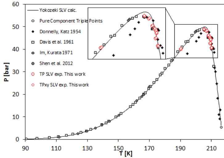
Figure 3. Comparison among literature data for the TP SLV locus of the \text{CH}_4\text{-CO}_2 mixture, experimental data obtained in this work and results obtained with the Yokozeki EoS [49] for SLV calculation.
