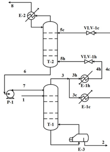
Figure 10. Process flow diagram for the new low-temperature distillation process [21].
