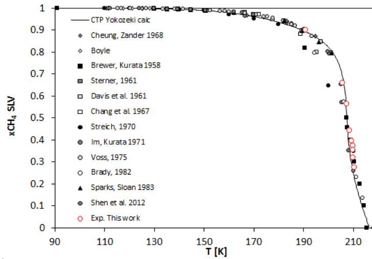
Figure 4. Comparison among literature data for the Tx SLV locus of the \text{CH}_4\text{-CO}_2 mixture, experimental data obtained in this work and results obtained with the Yokozeki EoS [49] for SLV calculation.
