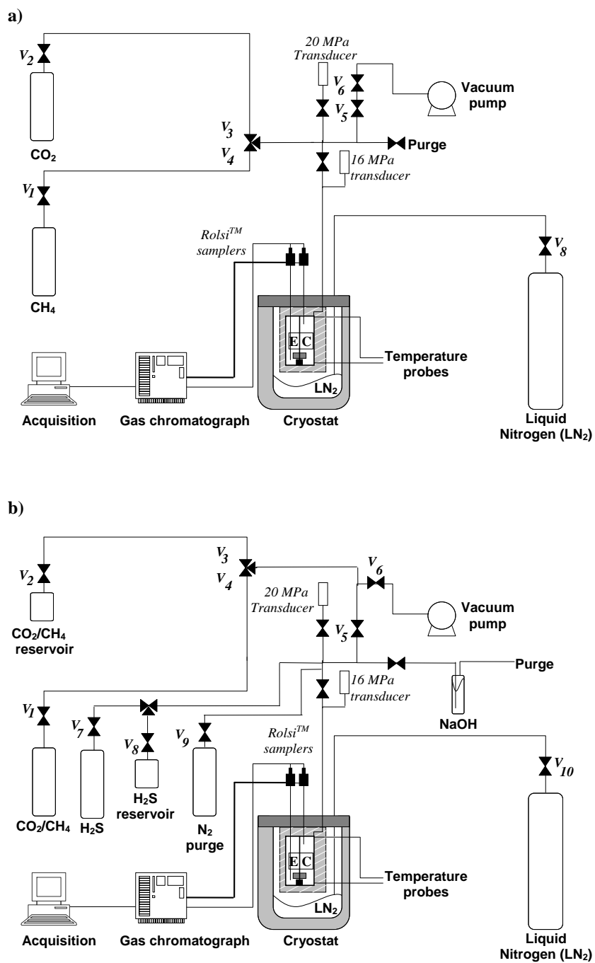
Figure 1. Flow diagram of the equipment used for a) TPxy solid apparition measurements for the CH 4 -CO 2 system and b) TPxy solid apparition measurements for the CH 4 -CO 2 -H 2 S system.
