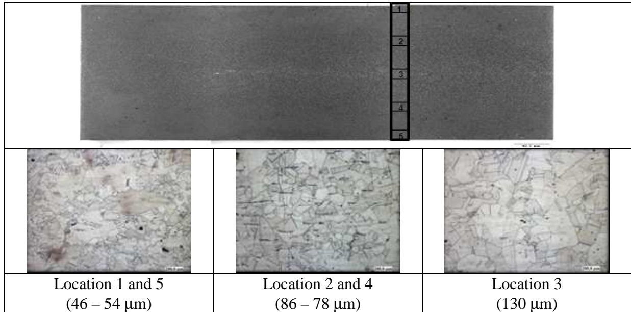
Fig. 3 : Microstructures through the thickness of the 155 mm plate (average grain size).
