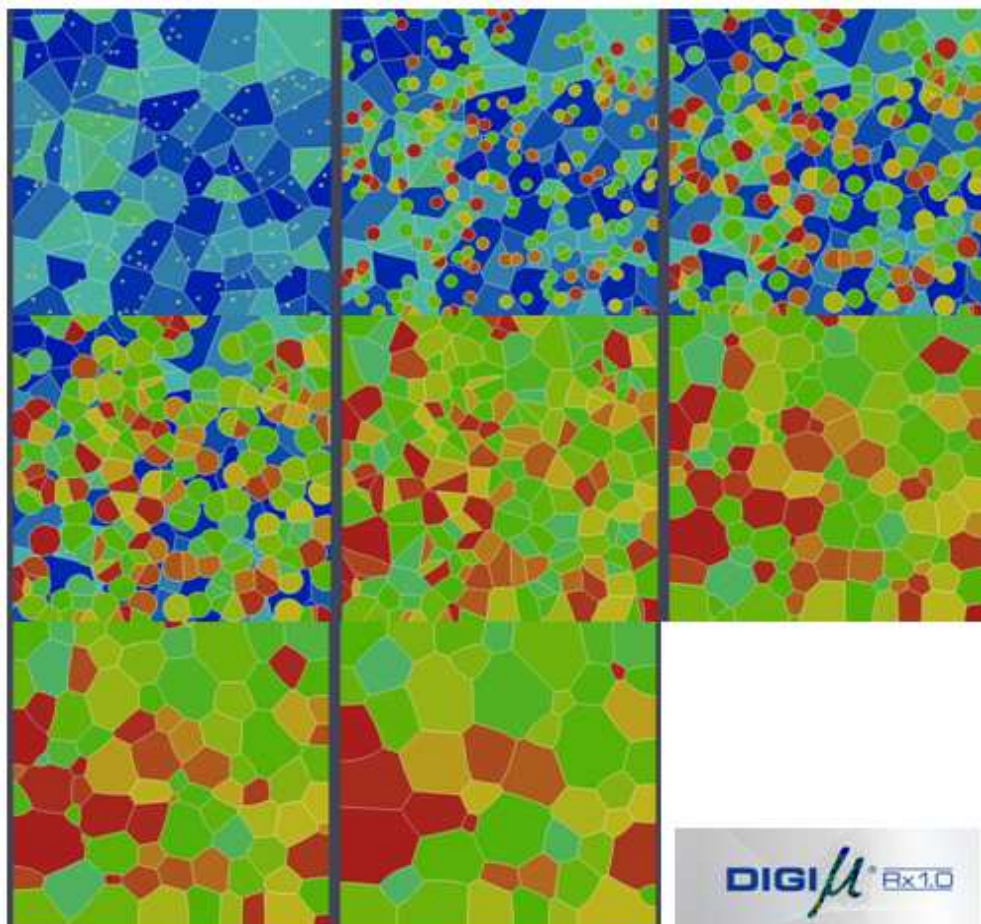
Fig. 8 : Modeling of site-saturated nucleation in 304L, from top to bottom and left to right : primary recrystallization and subsequent grain growth modeling [Fabiano, 2013].
