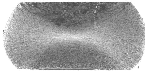
Fig. 1: Macro-etching after compression test on a 304 stainless steel sample.
