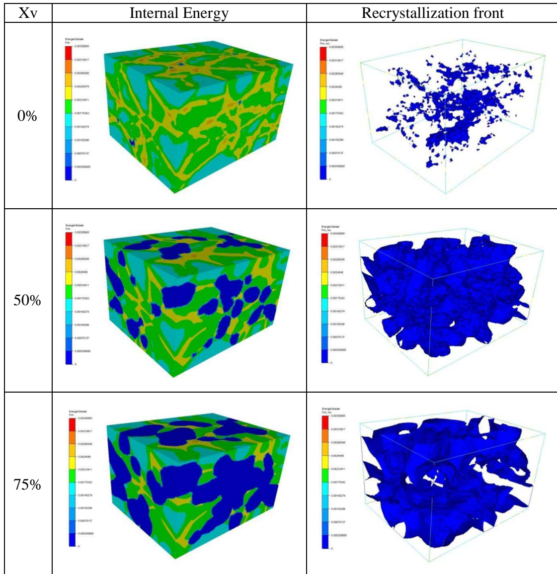
Fig. 9 : 3D recrystallization simulation based on CPFEM simulation results considering both statistically stored dislocations and geometrically stored dislocations (blue part corresponds to the ReX front) [Fabiano, 2013].
