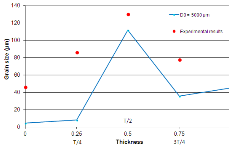
Fig. 4 : Comparison between results from Thermide model and observations.
