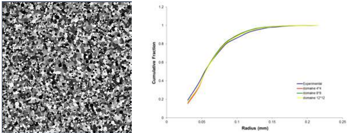
Fig. 7 : (left) A 2D digital microstructure made of 8294 grains obtained using a Laguerre-Voronoi method, based on a 304L steel experimental grain size distribution (domain size: 12 mm x 12 mm): (right) comparison between experimental grain size distribution and numerical ones for different size of REV.
