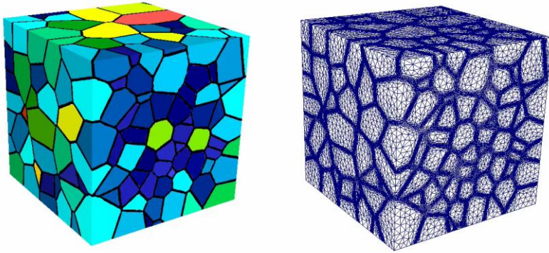
Figure 4: Polycrystal description in 3D with finite element mesh (anisotropic meshing near grain boundaries)
