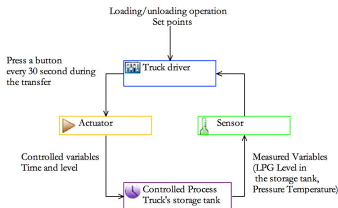
Fig. 2. Control structure
