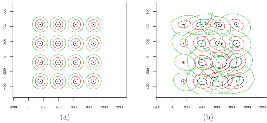
Figure 3: Covariance level contours at few points for the estimated stationary and non-stationary models (a, b). Level contours correspond to the values: 30000 (black), 20000 (red) et 10000 (green).
