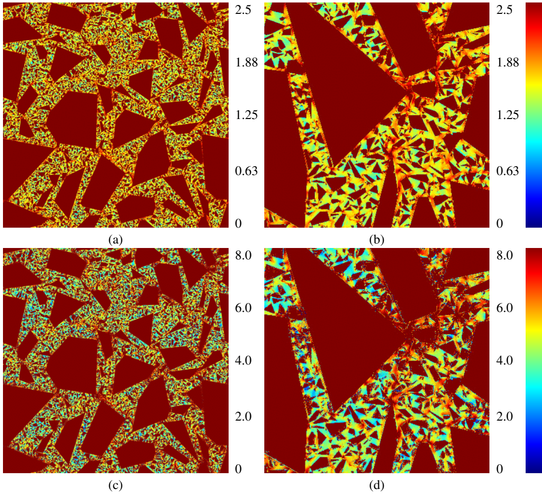
Figure 8: Maps of the normalized stress field \sigma_m / (E^c \epsilon_m) in the 3-scales model, for hydrostatic strain loading: contrast of properties \chi = 3 (a-b) and \chi = 100 (c-d). Maps (a) and (c): 1600^2 pixels, 14.4 cm 2D-sections, (b) and (d): 400^2 pixels, 3.6 cm enlargement. Color-scales are indicated on the right of each map.
