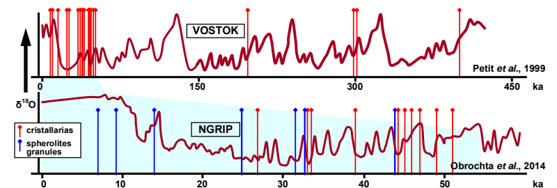
Figure 18 - Correlation of age estimations of the sand calcite in comparison to the time calibrated \delta^{18}O record of the VOSTOK 3 and NGRIP 4 ice core ^{18}O isotope curves. The sand calcites are bound distinctively to the cooling periods of the last four glacial periods. Analytical errors present \leq \pm 10\% .
