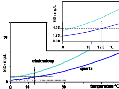
Figure 24 – Variations in quartz and chalcodony solubility with temperature (Bethke, 2002). The solubility of quartz decreases strongly when temperature decreases.
