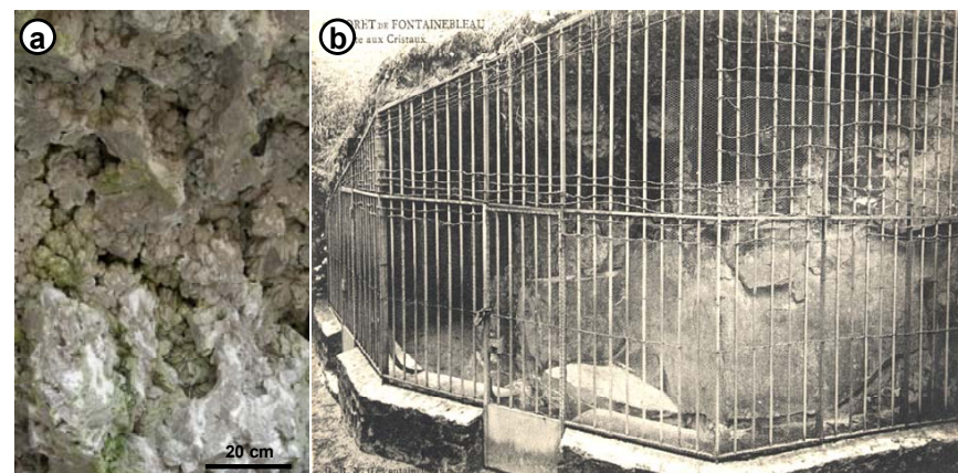
Figure 29 – Grotte aux Cristaux, Forêt de Fontainebleau (77). (a) "mutilated" calcite crystals at the roof of the cave, (b) the cave at the beginning of the XXth century with its strengthened protections (old post card).
