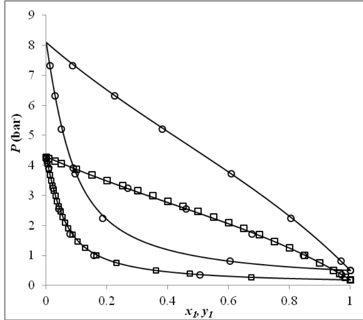
Figure 4. Isothermal P_{xy} diagram for the VLE of the diethyl sulfide (1) + n -butane (2) system. ( \circ ) Data measured in this work at 317.62 K and 343.14 K; ( \square ) Data from Dell'Era et al. [25] measured by the static-synthetic method at 317.60 K (vapor phase compositions were calculated through SRK EoS [21]); (—) calculated by Wilson model.
