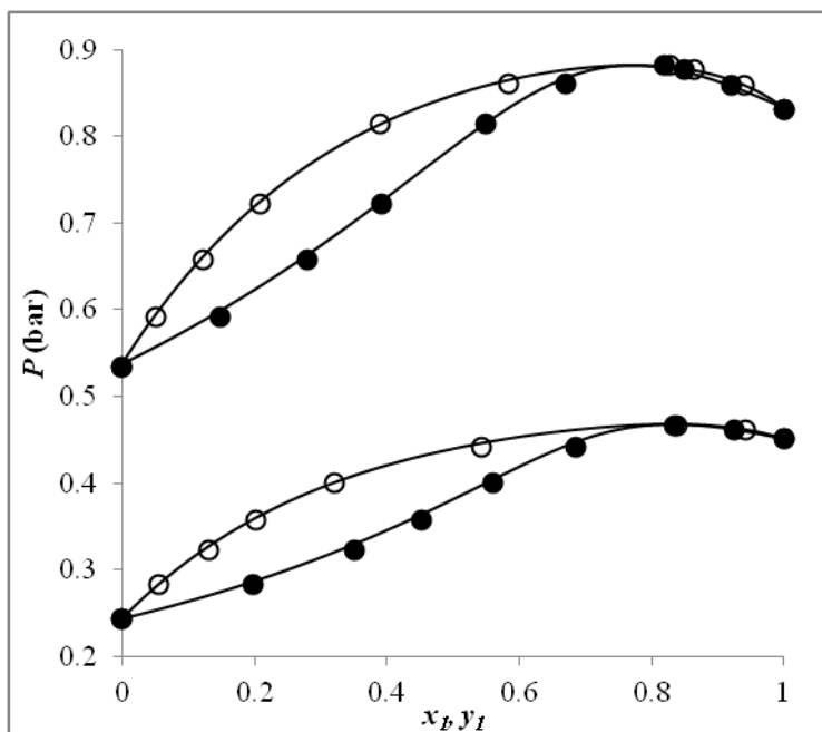
Figure 5. Isothermal Pxy diagram for the VLE of the 1-pentanethiol (1) + 1-pentanol (2) system. ( \circ, \bullet ) Data measured in this work at 372.75 K and 392.72 K; (—) calculated by Wilson model.
