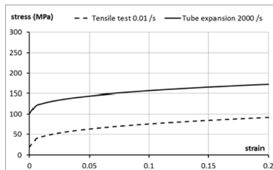
Fig.3. Stress-strain curves in quasi-static (0.01 /s) and dynamic (2000 /s) conditions.
