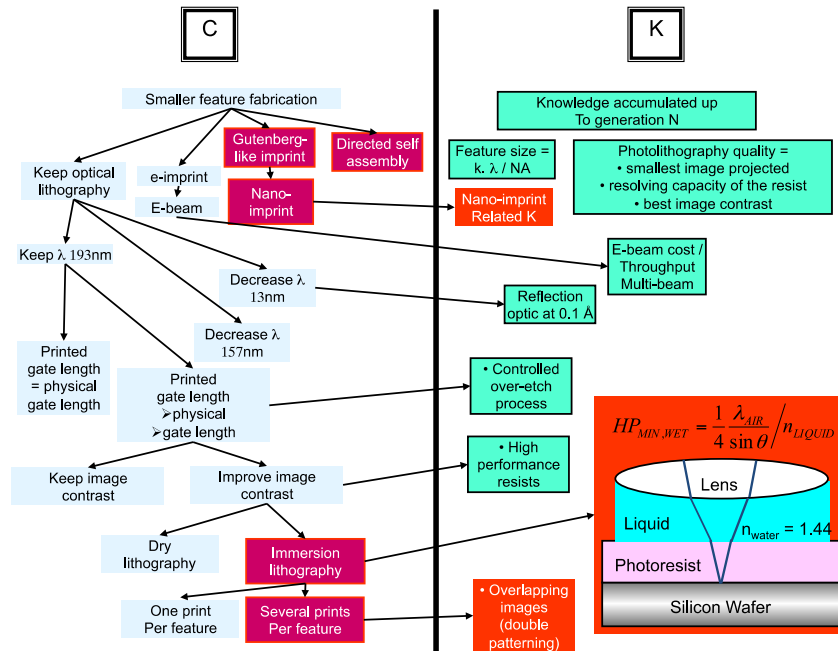
Figure 4: C-K referential of the ITRS roadmap for photolithography
