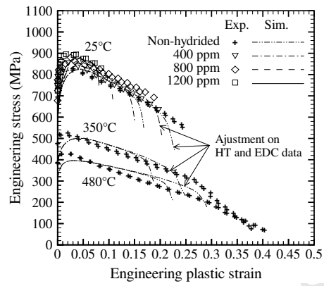
Figure 9: Experimental and calculated engineering stress–plastic strain curves for HT tests, for various temperatures and hydrogen contents. Results of calculations performed with parameters adjusted on HT and EDC tests data are included.
