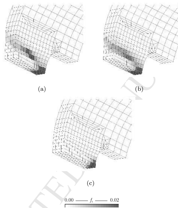
Figure 16: Total porosity fields calculated at crack initiation of PST specimens: (a) 25 °C, non-hydrated material, (b) 480 °C, non-hydrated material, (c) 25 °C, material hydrated at 1200 wt. ppm.
