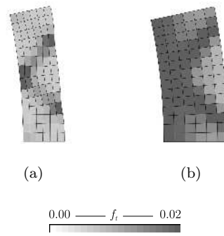
Figure 13: Total porosity fields calculated at crack initiation of EDC specimens tested at room temperature: (a) 25 °C, non-hydrated material, (b) 25 °C, material hydrated at 1200 wt. ppm.
