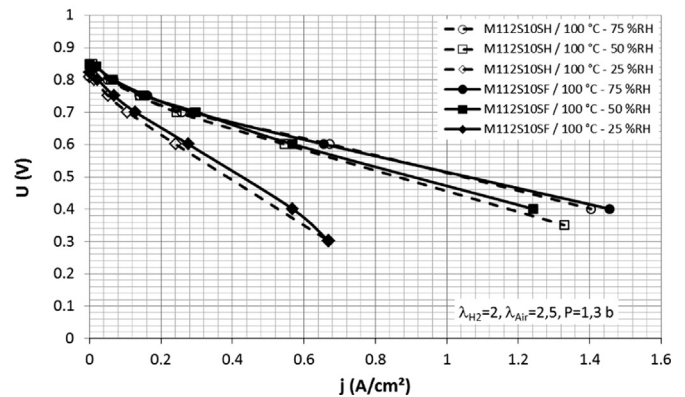
Fig. 14. Polarization curves obtained at 75 °C (up) and 100 °C (down) between 25% and 75% relative humidity for M112S10SH (dashed lines) and M112S10SF (solid lines).
