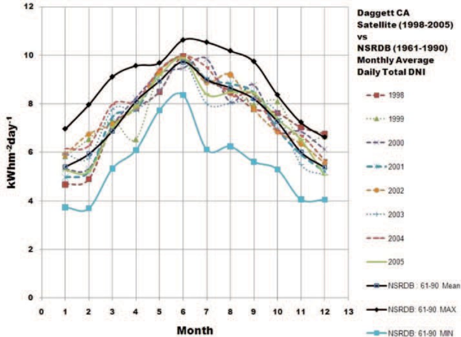
Figure 2-8. Example of direct-beam monthly average daily total (kWh/m 2 /day) interannual variability from 1961 through 2005 for Daggett, California. Data from Wilcox et al. (2007). Image from NREL
