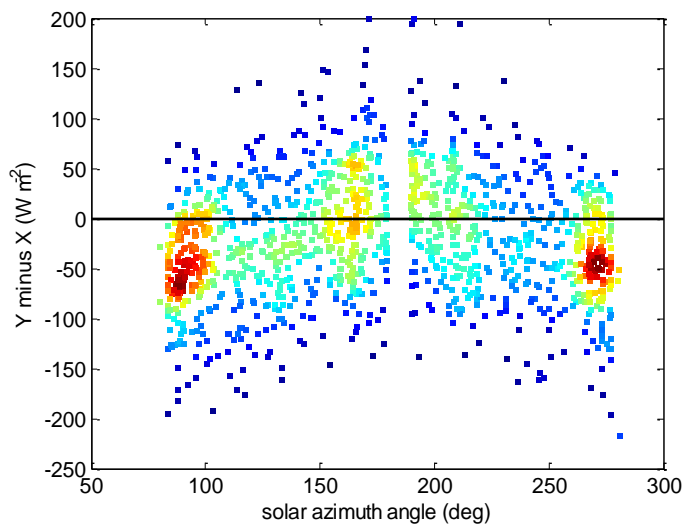
Figure 9. Residuals (McCleaar DNI minus ground measured DNI) versus the solar azimuth angle for Aswan under cloud-free conditions.
