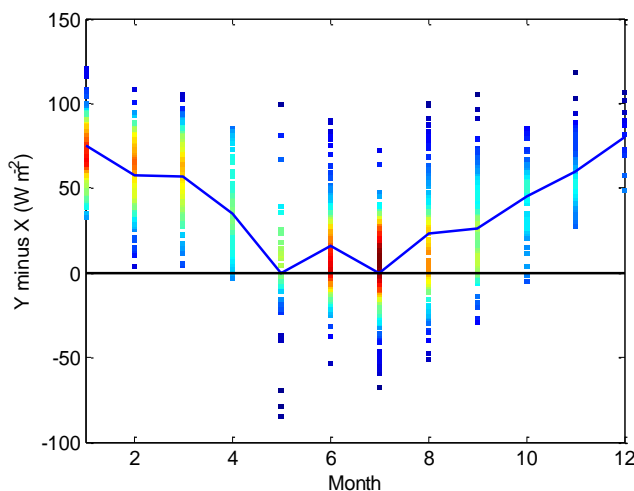
Figure 8. Residuals (McCleaar GHI minus ground measured GHI) versus the month for Aswan under cloud-free conditions. The blue line presents the monthly mean of the residuals.
