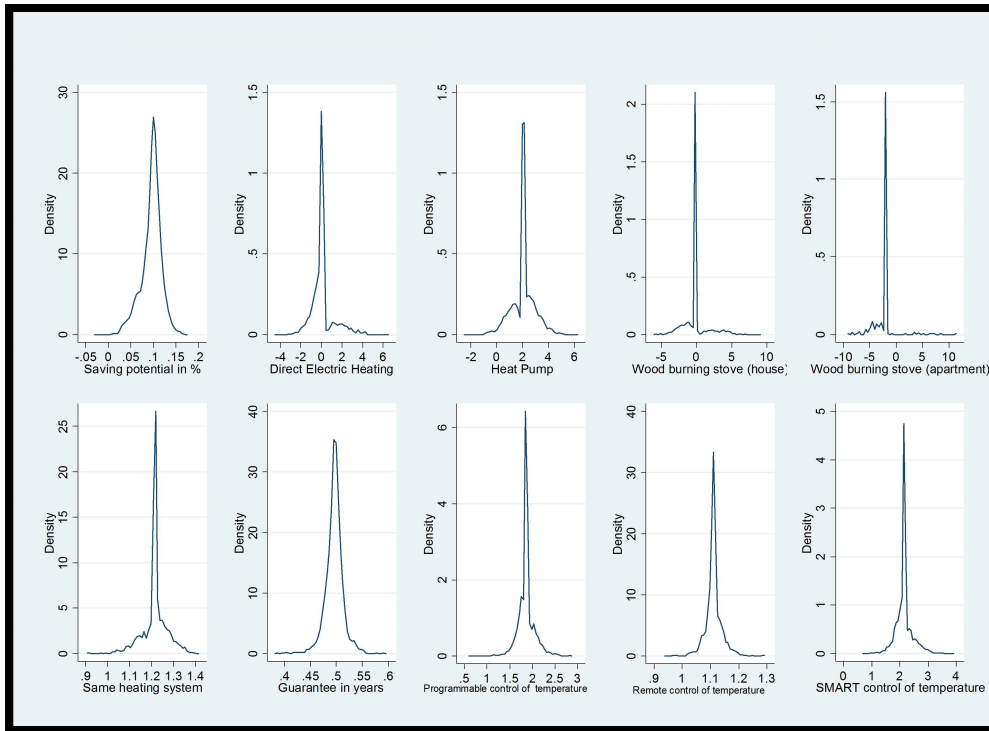
Figure 2: Kernel distribution of the individual-level coefficients (sub-situation 1, 1000 draws)
