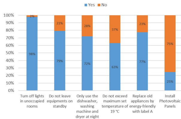
Figure 4: For each statement, do you agree?
