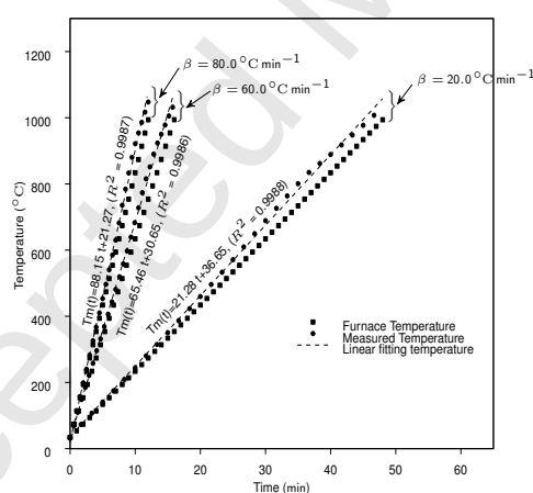
FIGURE 4: Variation of furnace and measured temperatures with respect to time at various heating rates : 20, 60 and 80 °C min -1
