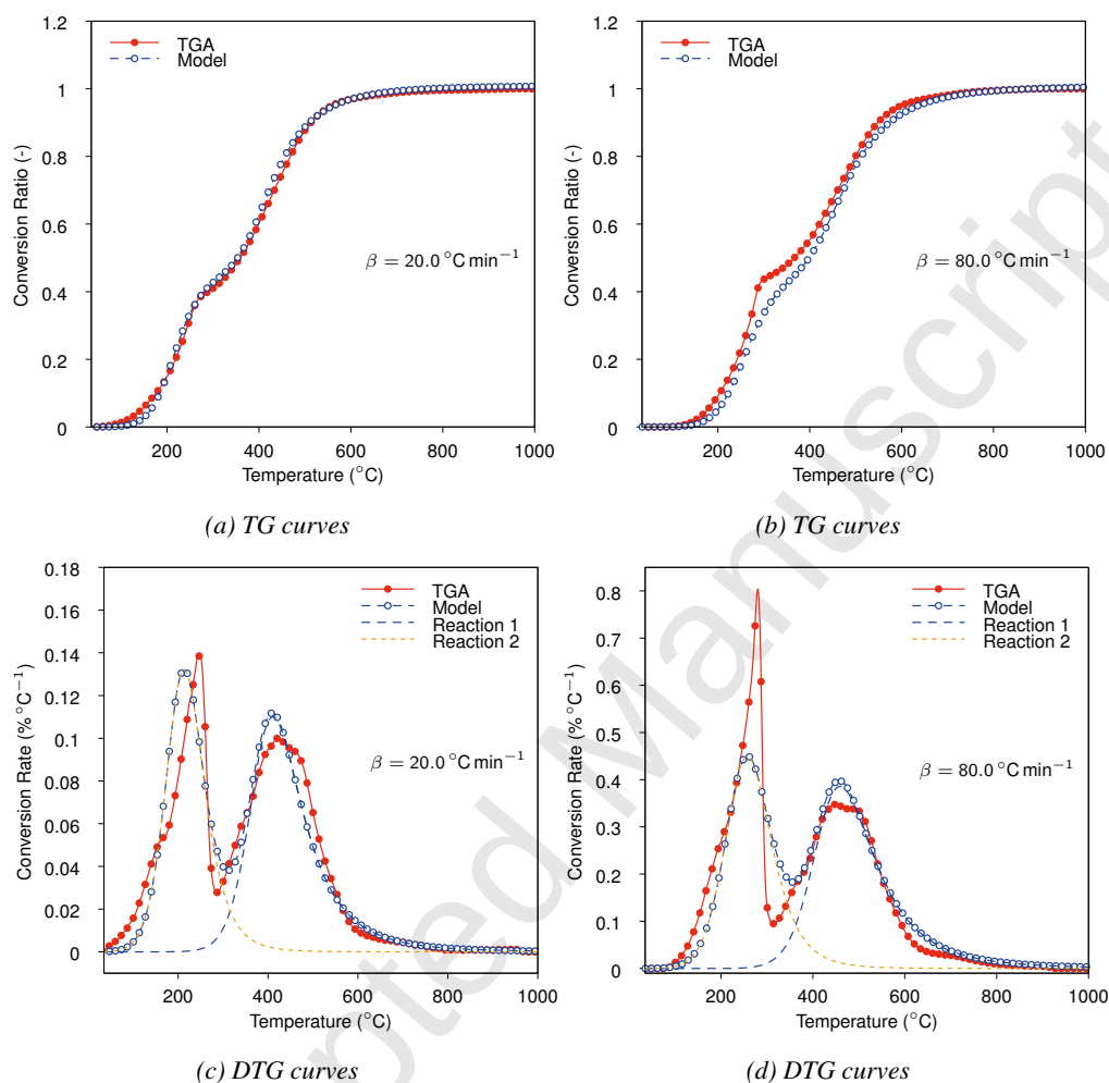
FIGURE 2: Experimental and calculated pyrolysis TG and DTG curves at the slowest and fastest heating rates, 20 and 80 ^\circ\text{C min}^{-1} , for 2-parallel independent reactions model
