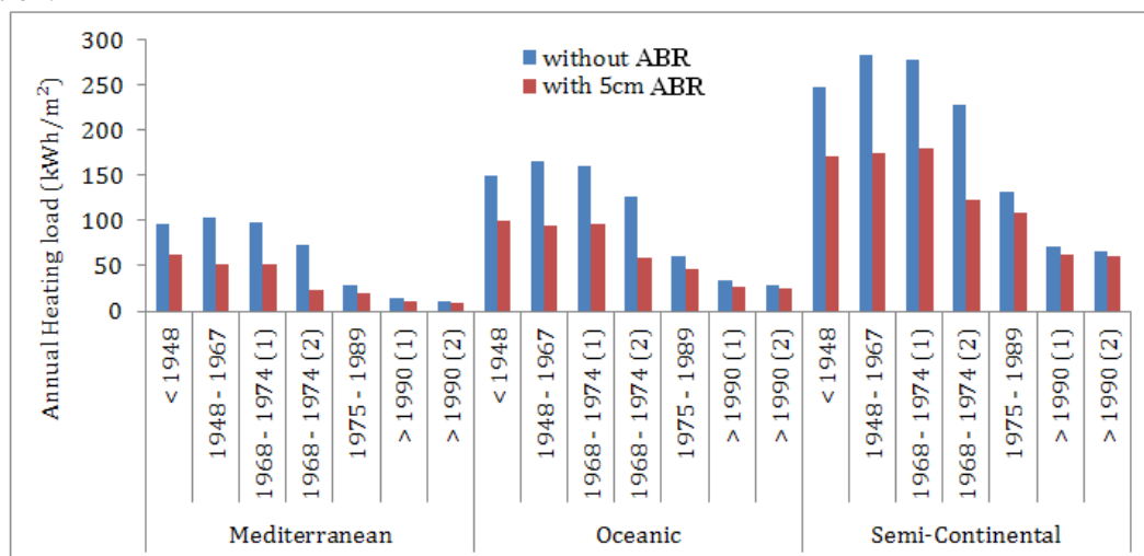
Figure 6: Annual heating load for the different climates and the different construction periods with and without the rendering
