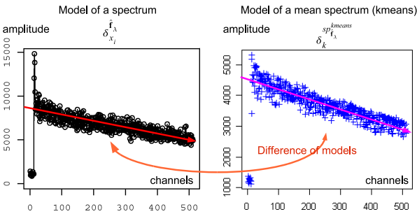
Fig. 16. Minimisation of the L_1 distance between the model of the mean spectra \delta_k^{sp_{\hat{\mathbf{f}}_\lambda}^{kmeans}} and the model of the spectra at each pixel \hat{\delta}_{x_i}^{\hat{\mathbf{f}}_\lambda} .
