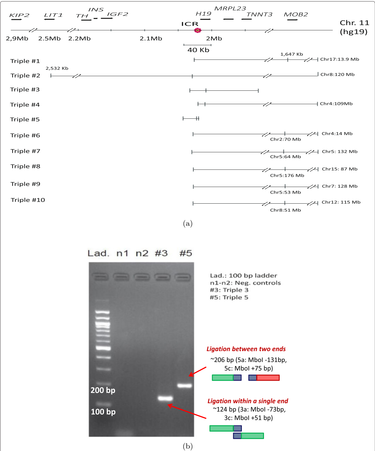
Figure 5 Validation of triples using PCR. (a) Ten triples extracted from the KBM7-TM3C-1 library that have at least one of their three ends in the 40 kb region surrounding the imprinting control region (ICR) of IGF2 and H19 genes. These triples involve short- and long-range contacts within chromosome 11 which are all indicated by tick marks with coordinates in kilobases (kb) displayed only for long-range contacts. Interchromosomal contacts with other chromosomes are indicated by the chromosome identifier followed by the coordinate in megabases (Mb). Orientation of the displayed locus is in the direction of IGF2 and H19 transcription. (b) PCR verification of pairwise contacts from triples 3 and 5. One pair of forward/reverse primers is used for each gel (Additional file 1: Table S1).
