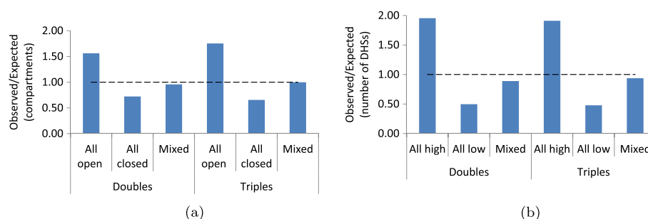
Figure 4 Genome-wide characterization of triple contacts. (a) Observed over expected percentages of double and triple contacts that link 1 Mb regions with the same (either open or closed) or different (mixed) compartment labels for the KBM7-TM3C-1 library (Methods). Both double and triple contacts prefer to link open compartments to each other with triples showing slightly more enrichment for this trend. (b) Similar percentages as in (a) but when 1 Mb windows are segregated according to the number of DHSs they contain (Methods). Contacts linking regions with higher numbers of DHSs than the median number are enriched within the doubles and the triples of the KBM7-TM3C-1 library. Due to lack of DNase data for KBM7 cells, we use data from six other human cell line for this analysis. Since the results are very similar among different cell lines, here we only plot the results for K562 which is also a leukemia cell line.
