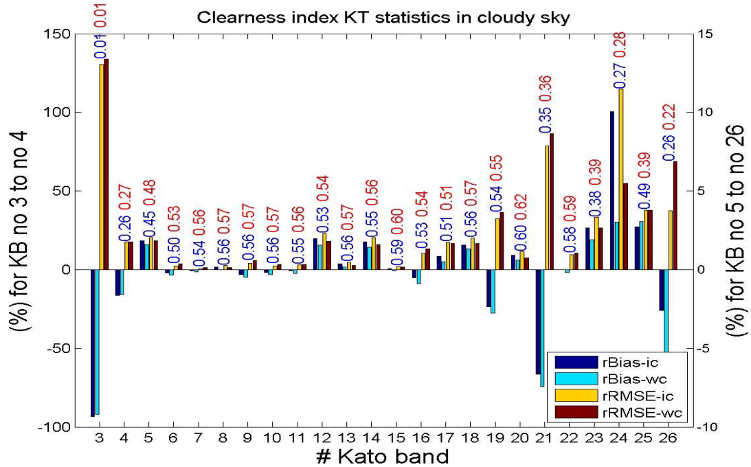
Figure 5: Synthesis of relative errors in each KB for the clearness index under cloudy conditions. Mean value of KT_i in each KB is reported in blue for ice cloud (ic) and red for water cloud (wc). Solar zenith angle less than 80^\circ .
