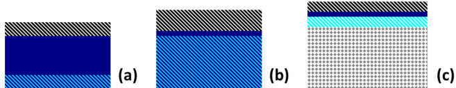
Figure 1: (a) Electrolyte supported cell (ESC), (b) Anode supported cell (ASC), (c) Metal supported cell (MSC).
