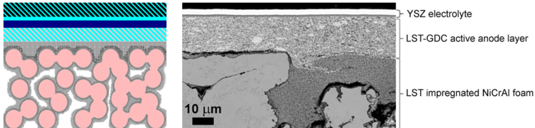
Figure 2: The EVOLVE cell, a metallic foam supported cell.
