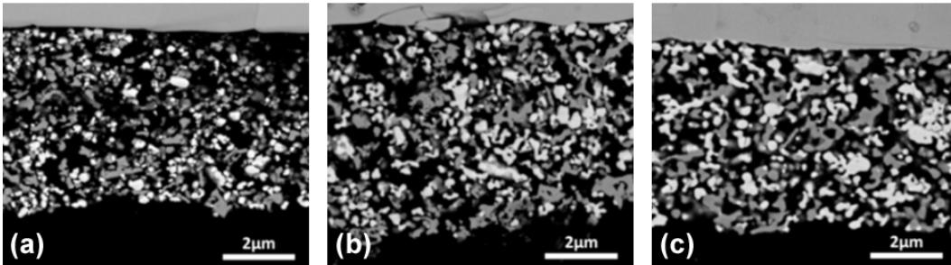
Figure 4: (a) LST – GDC10 and (b) LST – GDC20 sintered at 1000°C for 5 hours, (c) LST – GDC20 sintered at 1100°C for 5 hours.
